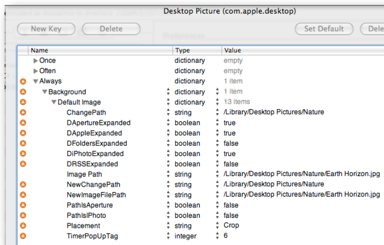
The final settings with empty settings deleted
