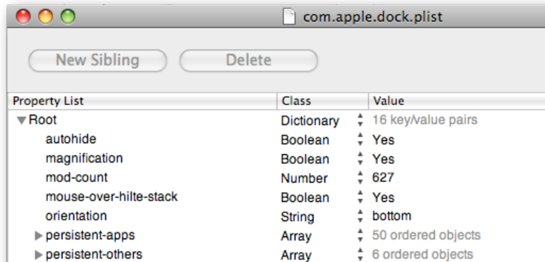
Local user's Dock settings viewed from Property List Editor
