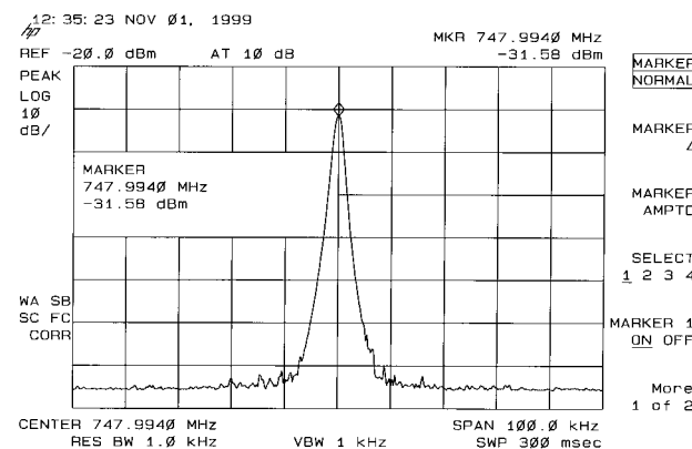
FIGURE 9. IF LOCAL OSCILLATOR OUTPUT (TEST POINT H)
