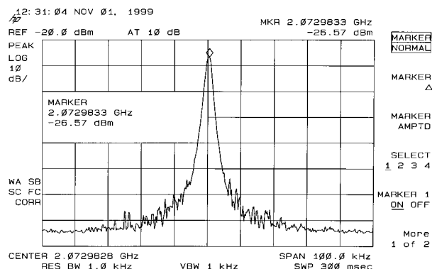
FIGURE 8. RF LOCAL OSCILLATOR OUTPUT AT CHANNEL 8 (TEST POINT F)
