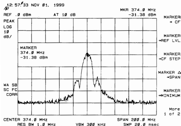
FIGURE 5. IF TRANSMIT SIGNAL BEFORE SAW FILTER (TEST POINT C)
