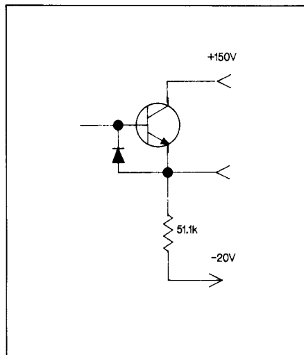
Figure 1. Original series regulator circuit.
