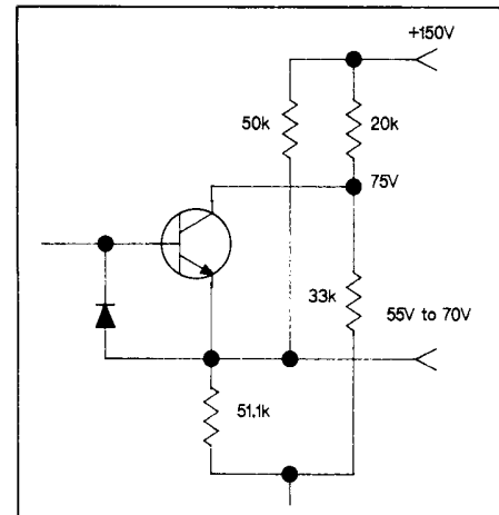
Figure 2. Simard's modification of Figure 1 to reduce the power dissipation through the transistor.
