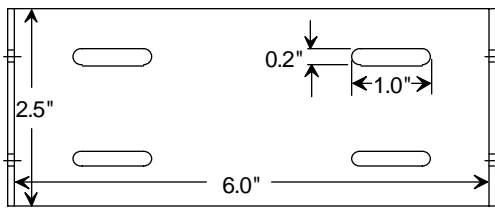
Figure 1 - Mounting plate and slot dimensions
