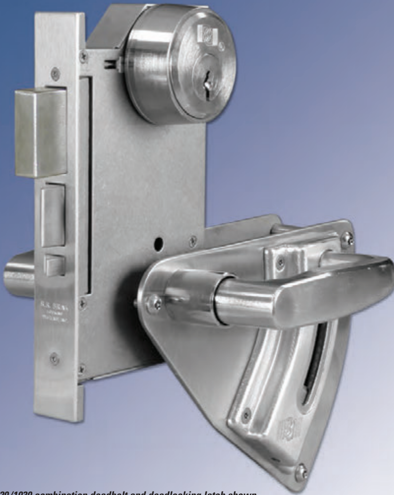
1020/1030 combination deadbolt and deadlocking latch shown with R.R. Brink Mogul key cylinder, and Lever Eskort
