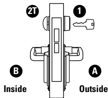
ANSI F13 Dormitory or Exit Lock
