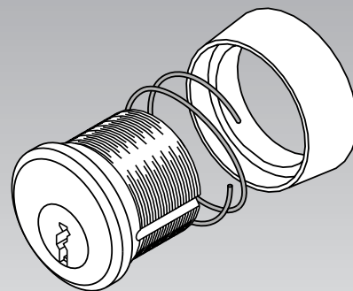
RRBS proprietary "Mogul" (MOG) key cylinder can be specified.
