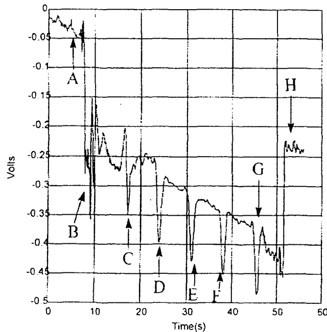
Figure 2. Respiration signature taken by RADAR Flashlight through a 8 inch hollow core concrete wall
