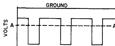
Figure 10. Voltage across the INTERP terminals.
