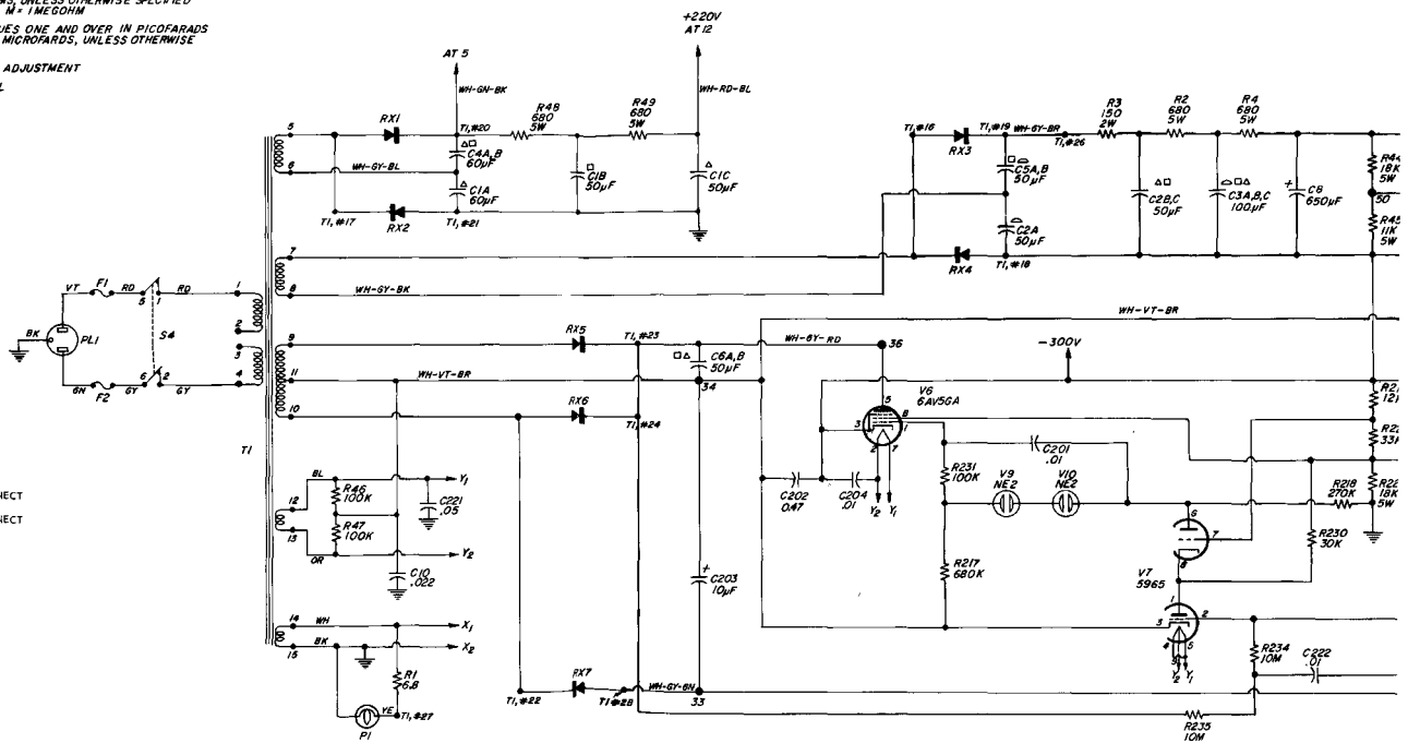
Figure 25a. Schematic diagram. (See also Figure 25b)
