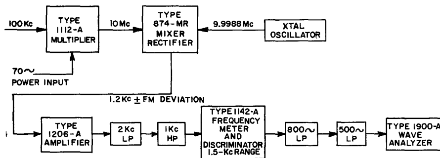
Figure 17. Setup Used to Measure FM Noise Level of Type 1112-A Standard-Frequency Multiplier.
