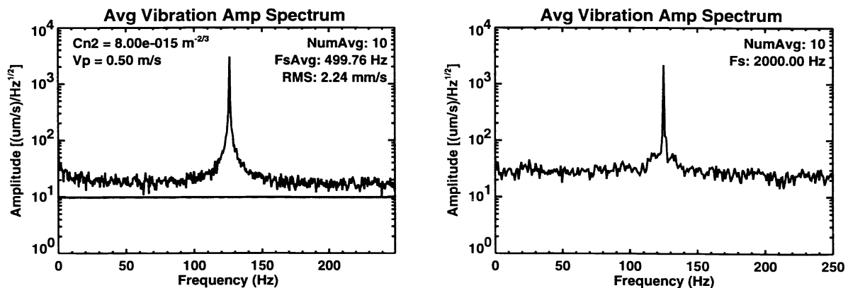
Figure 11: CW and doublet-pulse vibration spectra of a calibration target.
