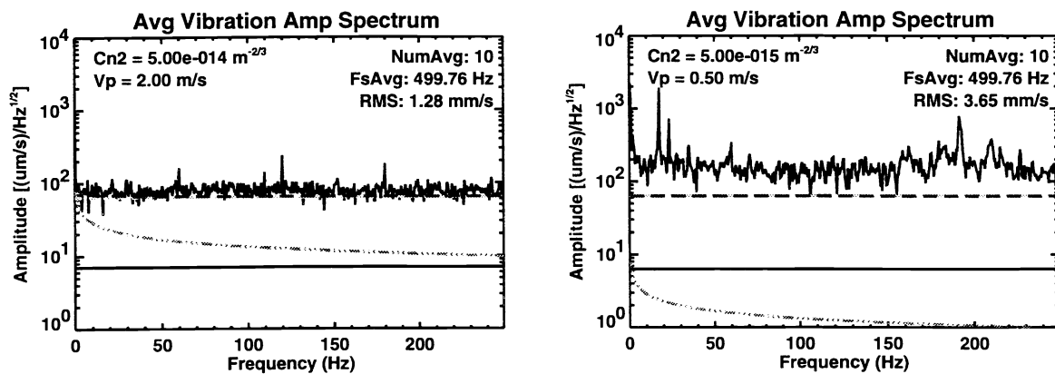
Figure 13: Doublet-pulse vibration spectra of the engine of a Honda Accord at 7.5 km.
