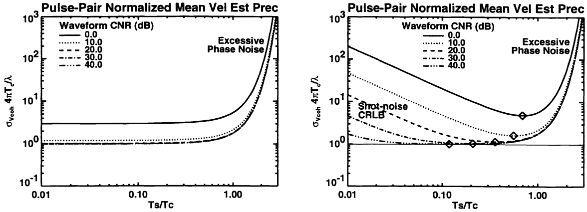
Figure 5: Velocity estimate precision for the doublet-pulse waveform
