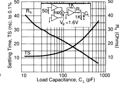
Settling Time vs Capacitive Load, A_{VMAX} = \pm 10
