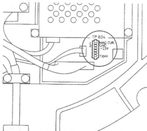
Fig.43 Measuring the Magnetron Current
