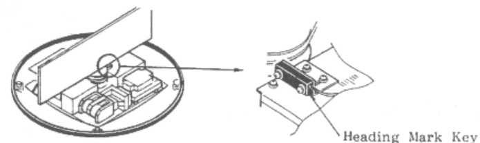
Fig.13 Location of Heading Mark Key
