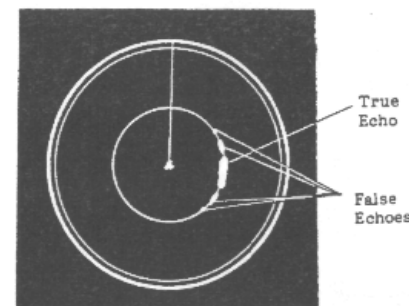
Fig.33 Side-Lobe Echoes
