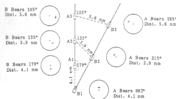
Fig.40 Relative Motion vs. True Motion
