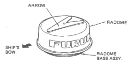
Fig.8 Radome Cover Placement
