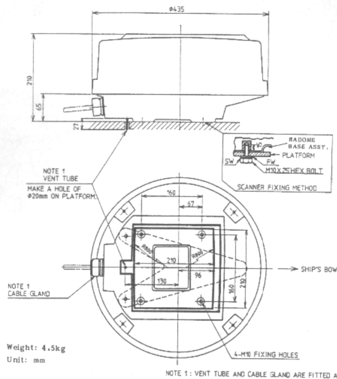
Fig.6 Scanner Unit Outline Drawing
