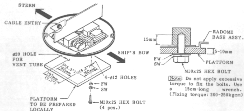
Fig.5 Installing the Scanner Unit
