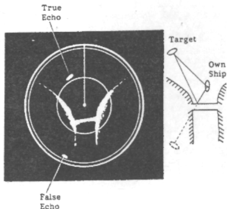
Fig.35 Indirect Echoes
