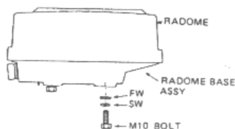
Fig.3 Preparing the Radome Base for Mounting
