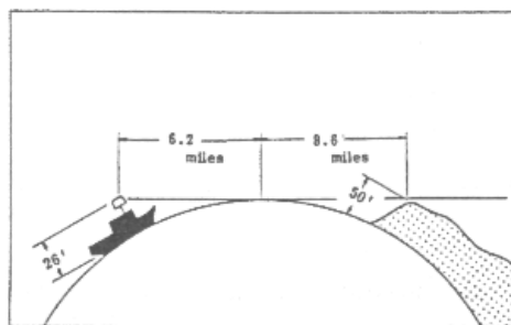
Fig.30 Radar Horizon
