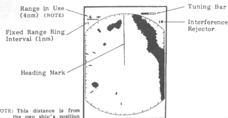
Fig.20 Location of Display Screen Indicators
