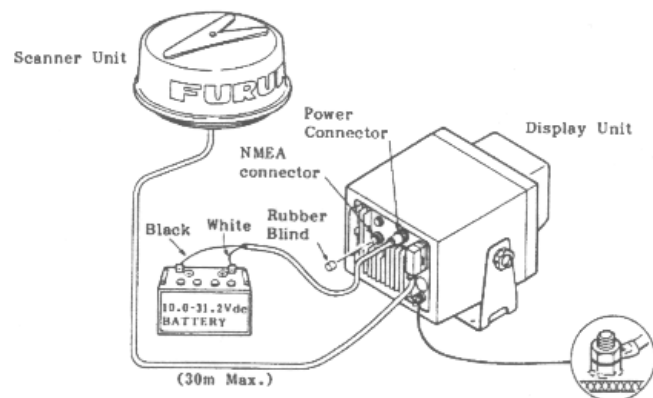
Fig.11 Detailed Wiring Diagram
