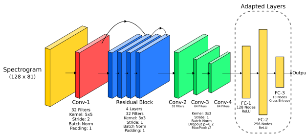
Fig. 11: Architecture of speech classification network.
