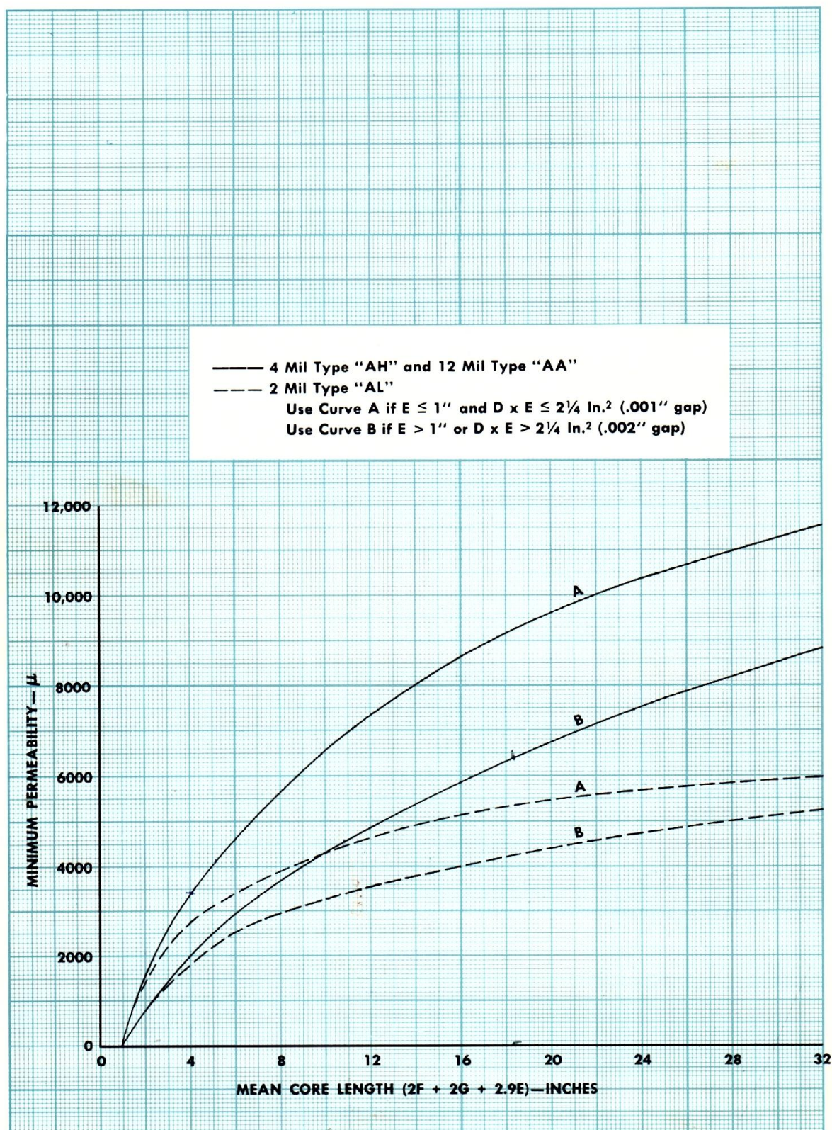
FIG. 12—MINIMUM DESIGN PERMEABILITY FOR SILELECTRON "C" CORES AT 60 CPS, 10 KILOGAUSSSES
