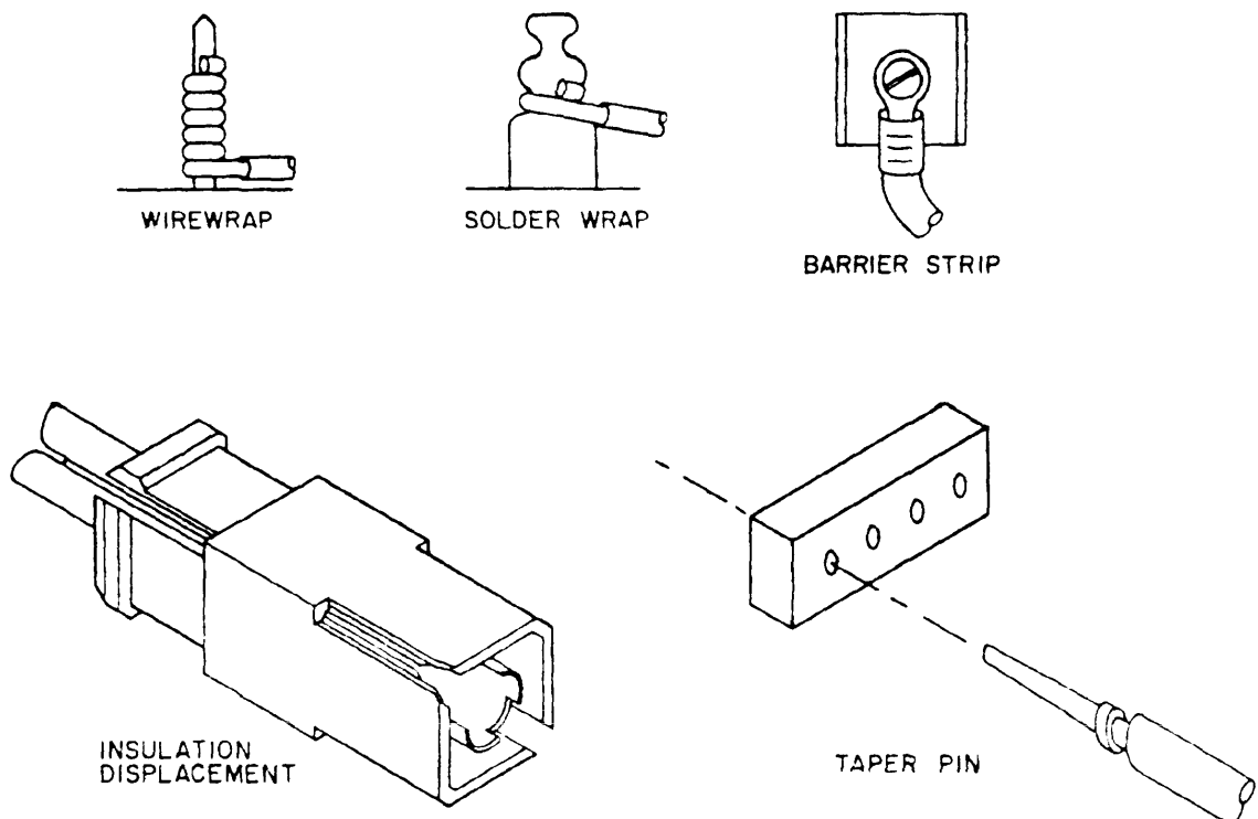
FIGURE 30. Termination techniques.
