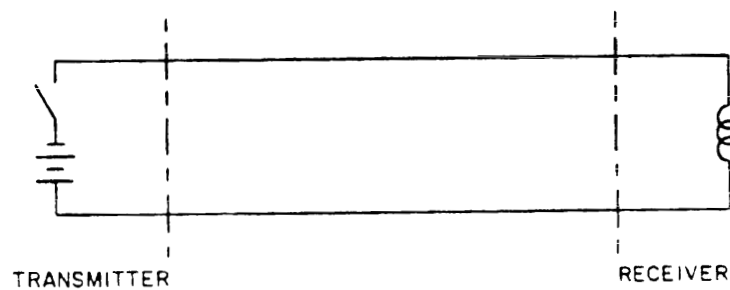
FIGURE 37. Loop current.
