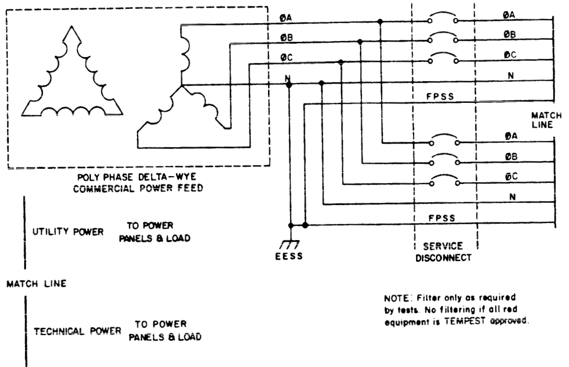
FIGURE 21. Dedicated transformer feed.
