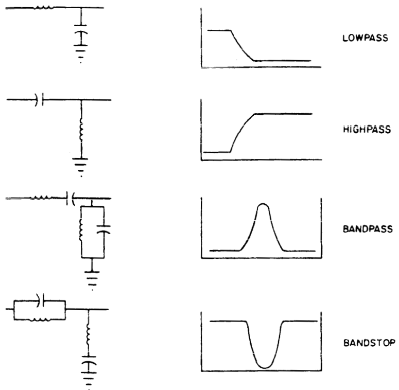
FIGURE 44. Filter action.
