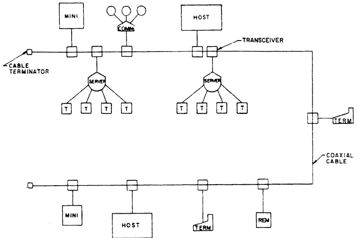
FIGURE 7. Multipoint topology.
