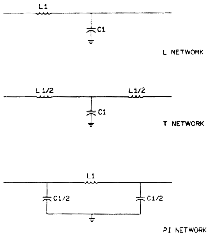
FIGURE 45. Filter construction.
