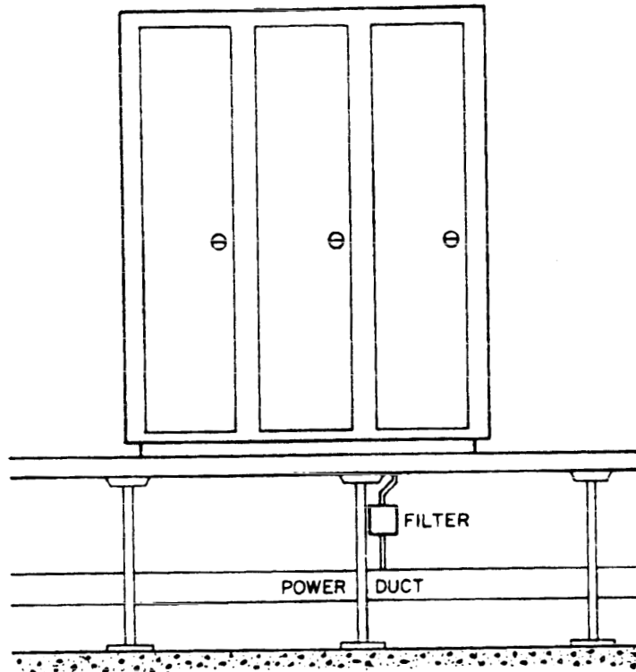
FIGURE 46. Equipment filtering, preferred method.
