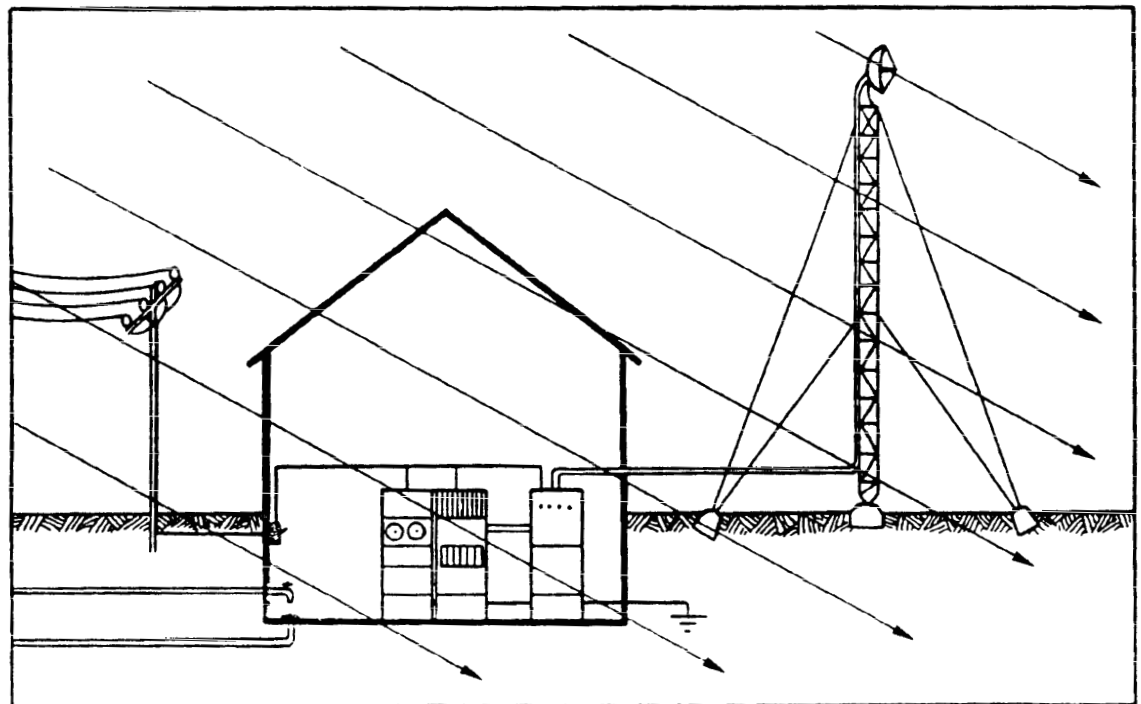
FIGURE C-4. Protection principles.
