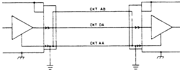
FIGURE 38. RS-232C interface.
