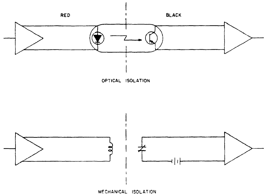
FIGURE 42. Isolator techniques.
