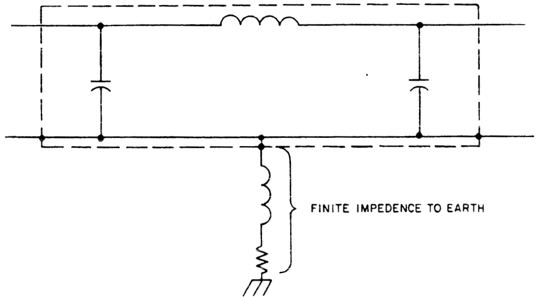
FIGURE 9. Typical signal or power-line filtering.
