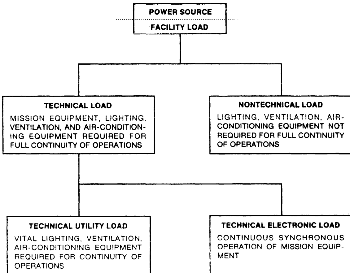
FIGURE 2. Power distribution.
