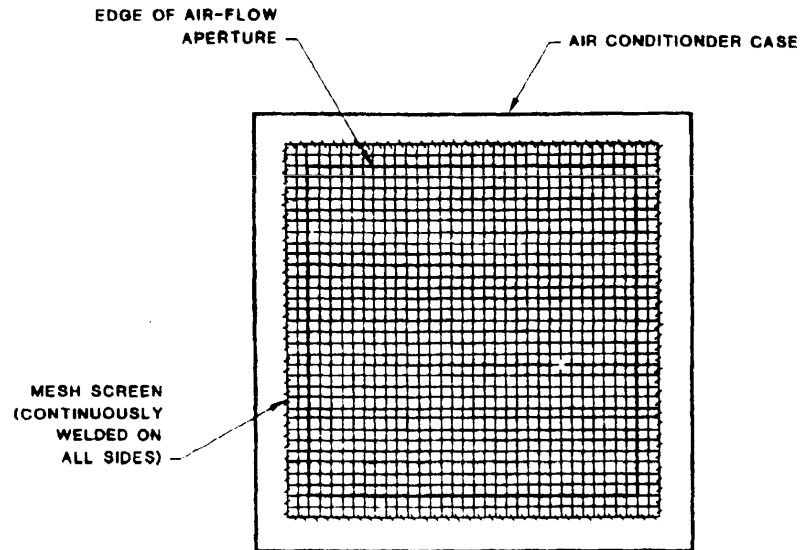
FIGURE A-8. EMP/HEMP protection screen for air-conditioner apertures.
