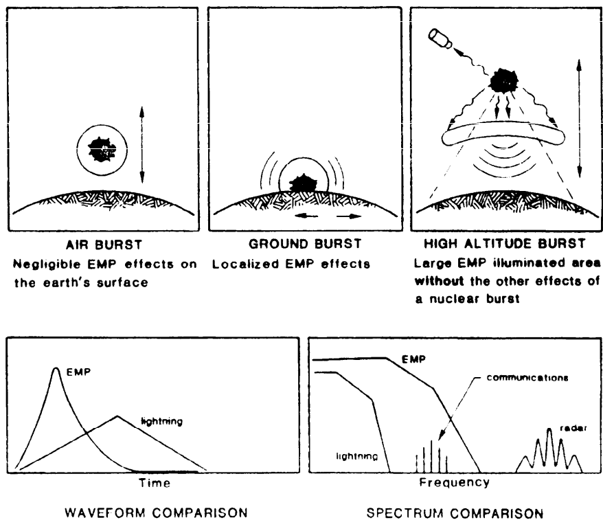
FIGURE C-2. EMP characteristics.
