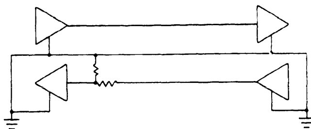
MIL-188-114 UNBAL TO RS-232
