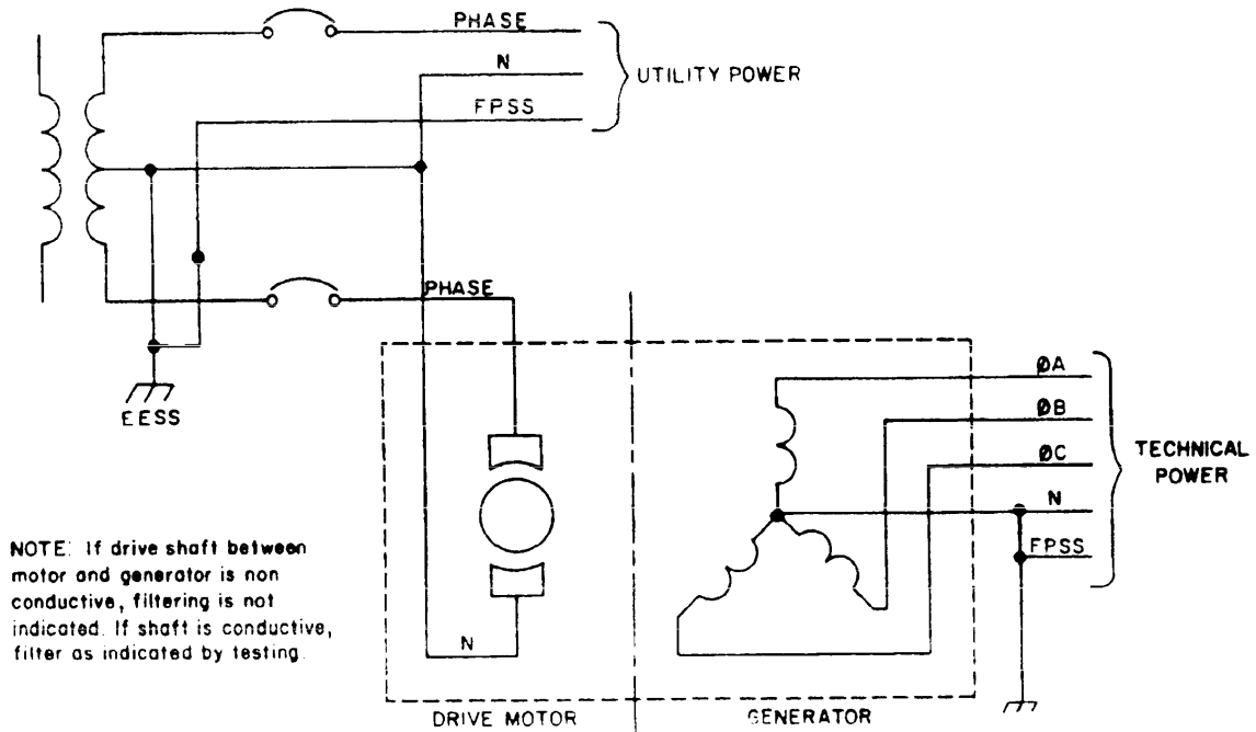
FIGURE 18. Motor generator.
