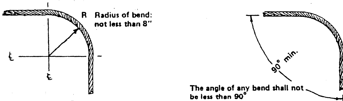
Figure 5. Radius and Angle of Down Conductor Bends
