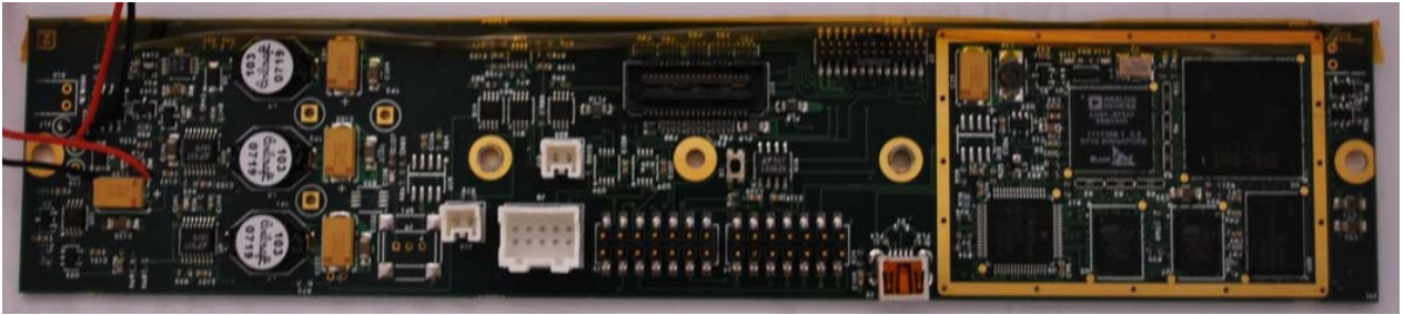
Figure 5: RANGE-R DSP PCB Front
