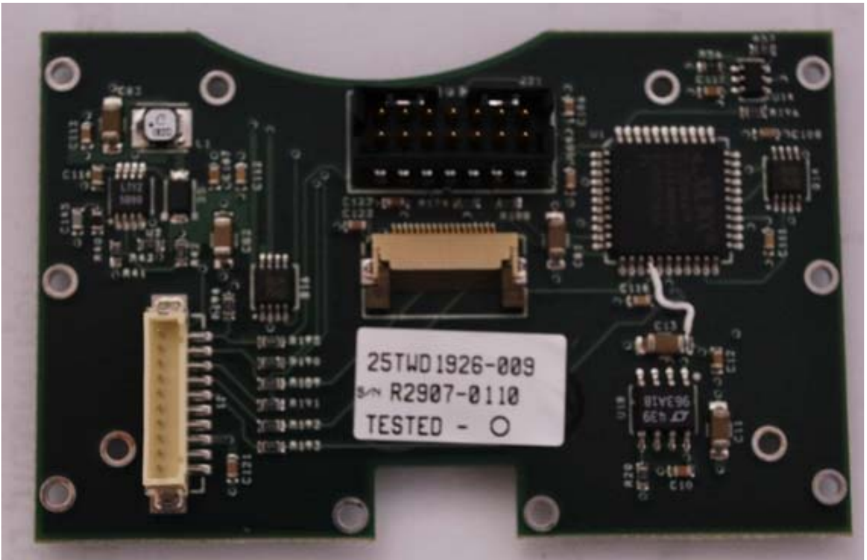
Figure 7: RANGE-R Display PCB Front
