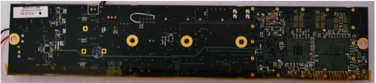
Figure 6: RANGE-R DSP PCB Back
