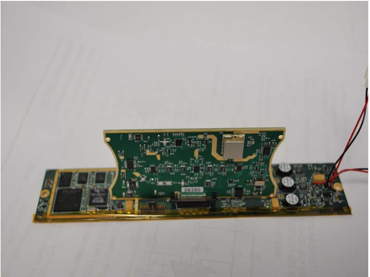
Figure 2: RANGE-R RF-DSP CCA Assembly
