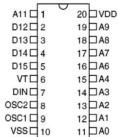
HT604L – 20 DIP/SOP
