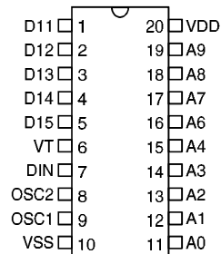
HT605L – 20 DIP/SOP
