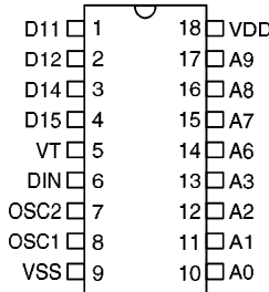
HT694 – 18 DIP
