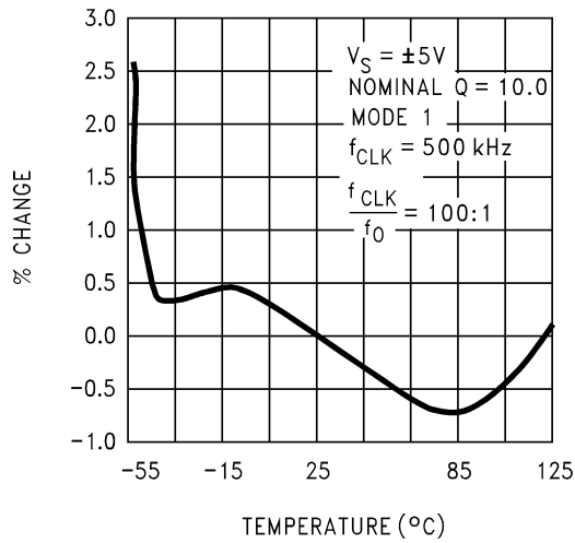
Q Deviation vs. Temperature
