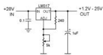
Adjustable Positive Voltage Regulator
