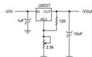
Adjustable Negative Voltage Regulator
