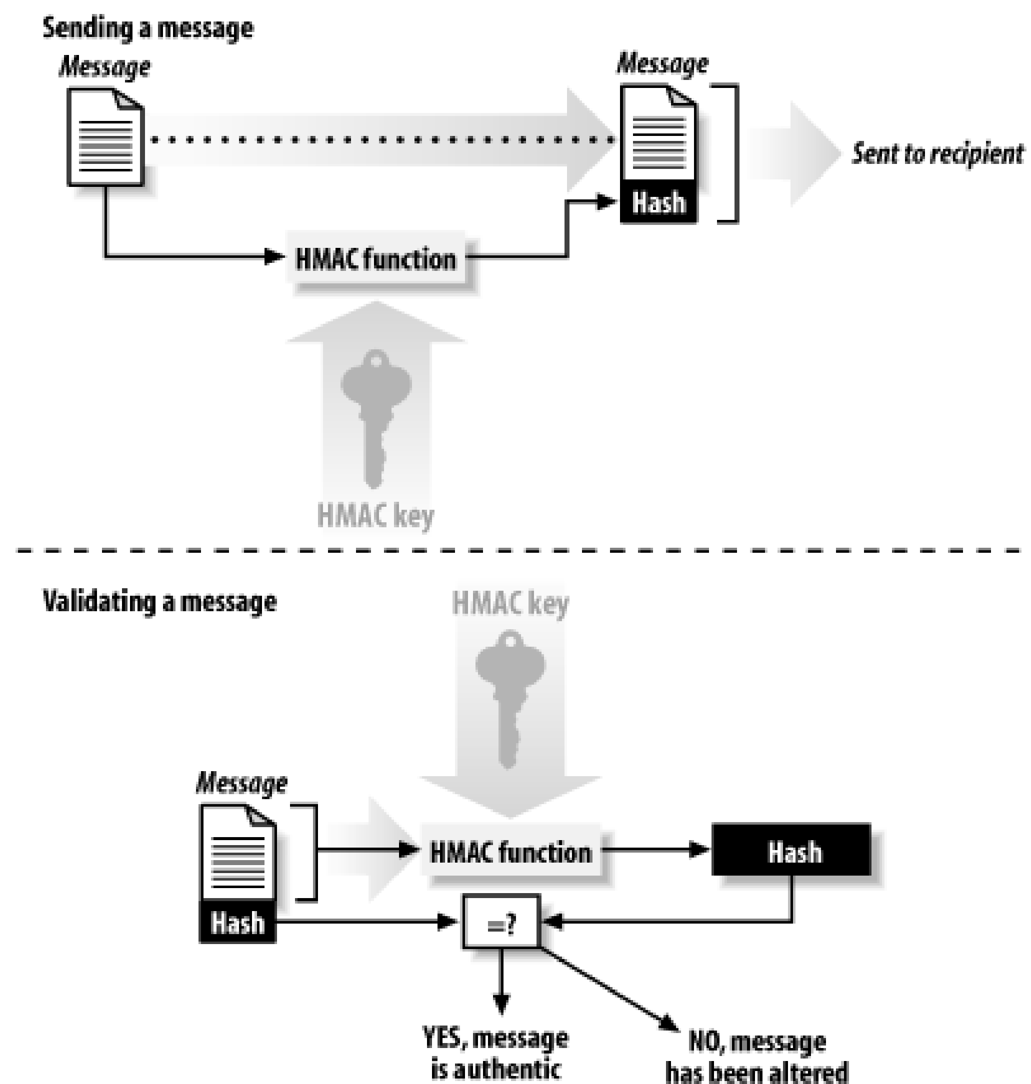
Figure 7-5. Using an HMAC to verify the authenticity and integrity of a message
