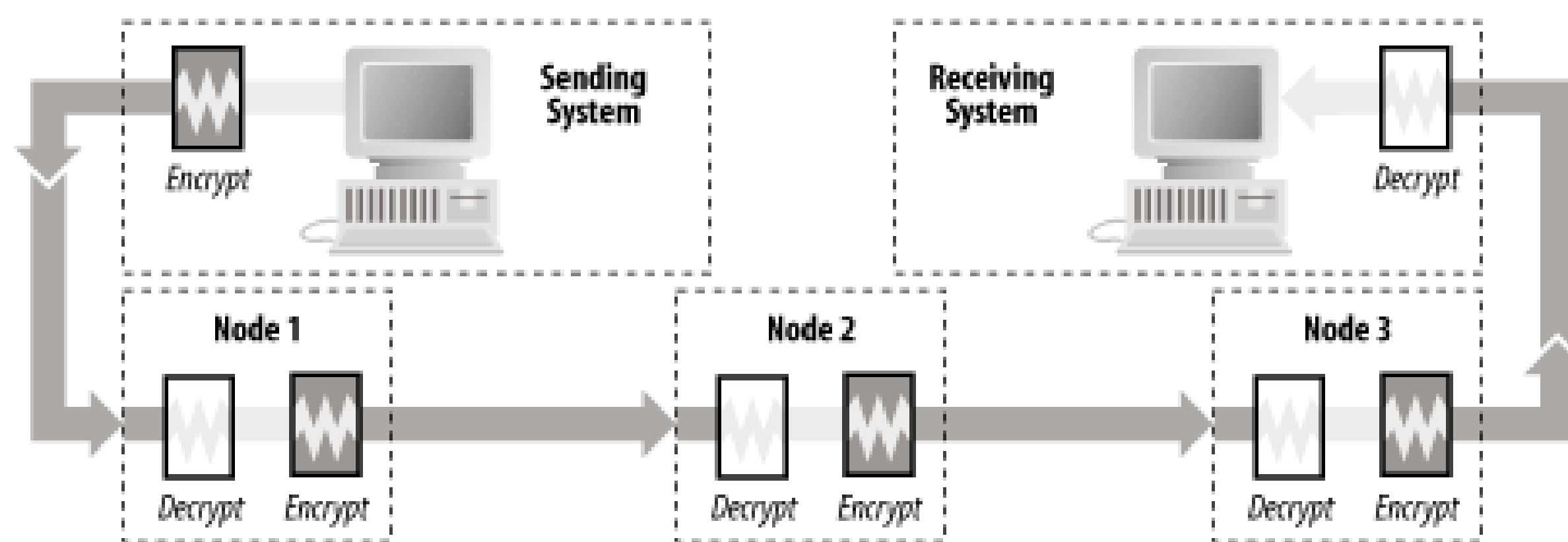
A Link Encryption
