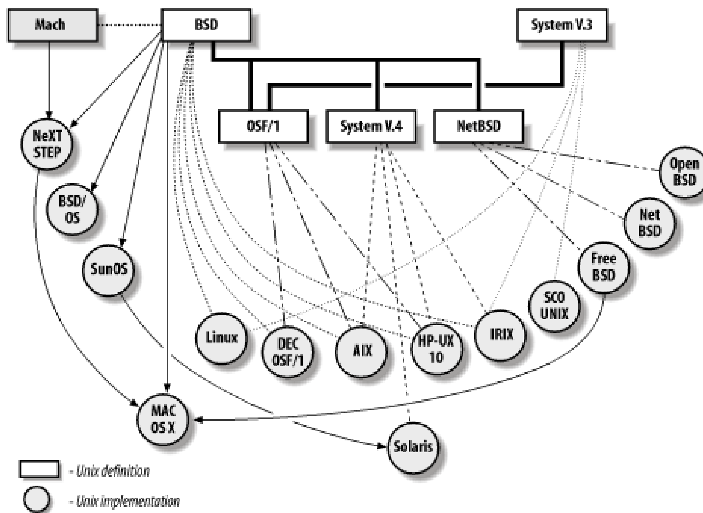
Figure 2-1. Unix variants
