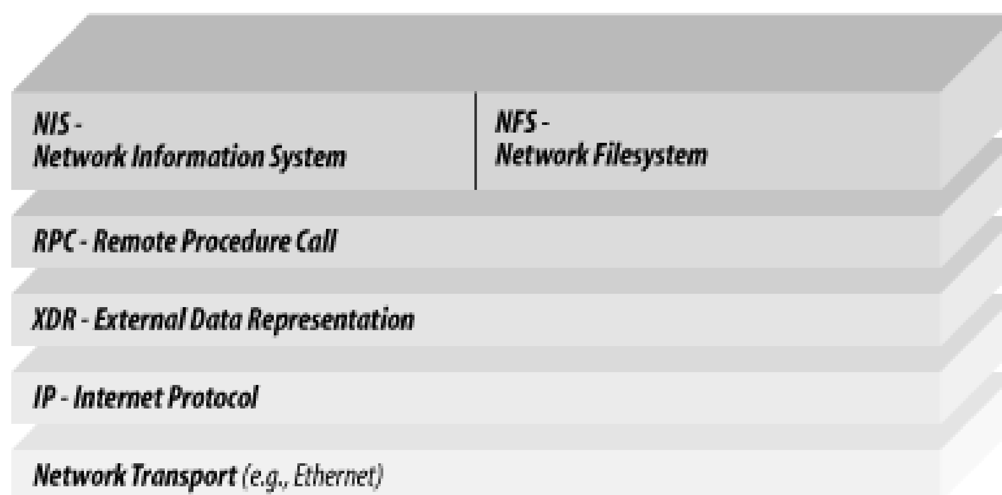
Figure 15-1. NFS protocol stack
