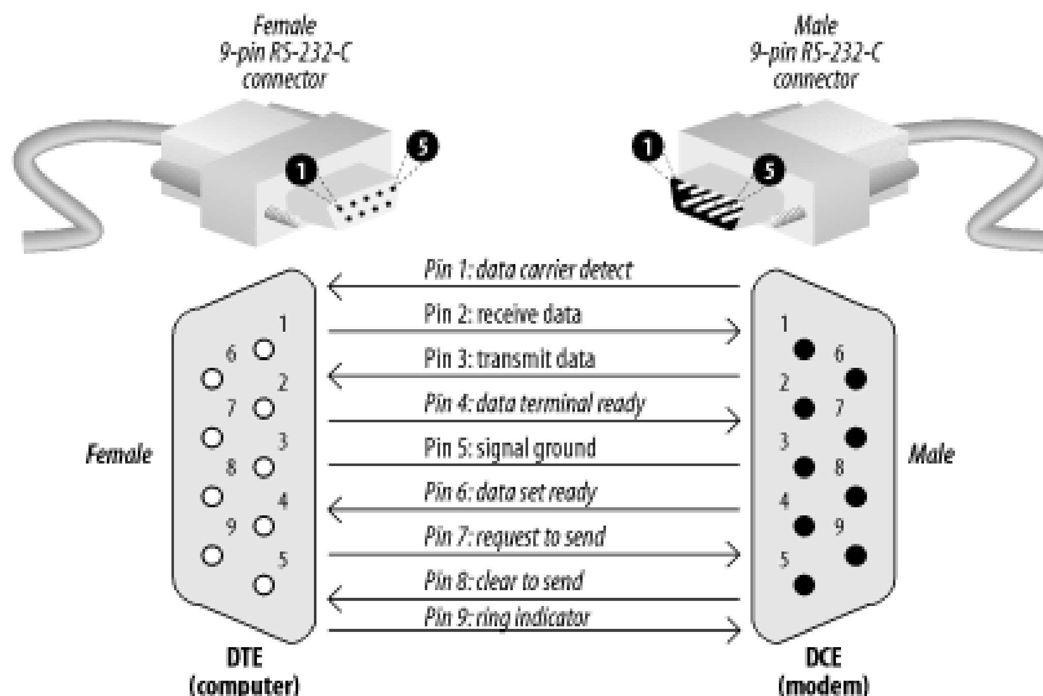
Figure 10-3. The standard 9-pin RS-232-C connector
