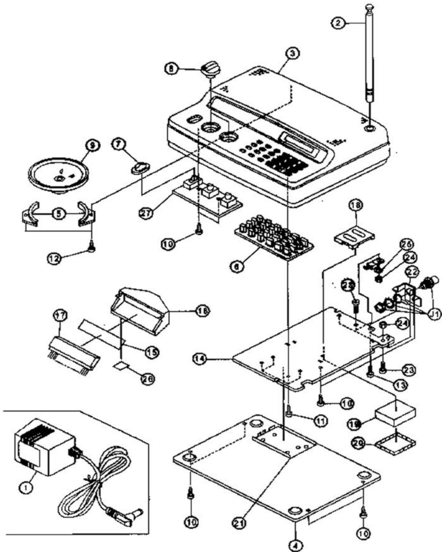
MODEL PRO-2018 200-CHANNEL DESKTOP SCANNER EXPLODED VIEW (200-0424) FAXBACK DOC # 12893
