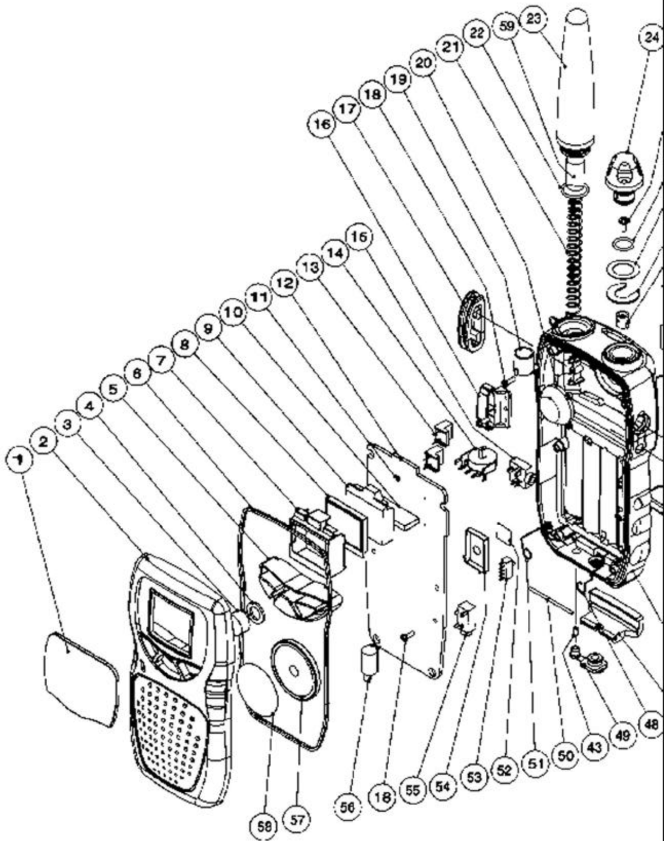
14-CHANNEL PERSONAL FRS 2-WAY RADIO WITH QUIET CODE EXPLODED VIEW (210-1864) SHEET 1 FAXBACK DOC # 12894
