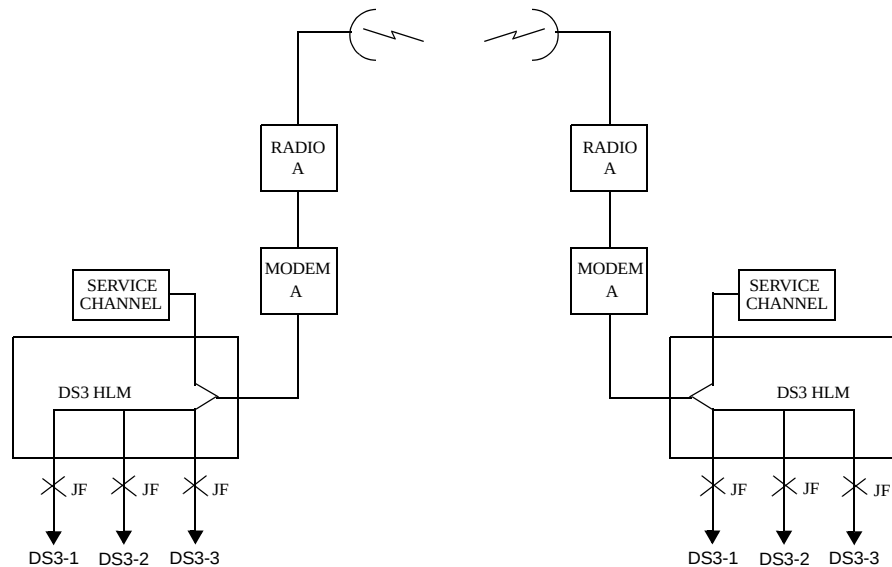
Figure 3-9: 3xDS3 to 3xDS3 configuration
