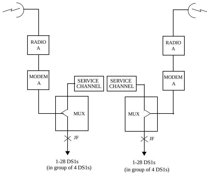
Figure 3-4: Multiplexer configuration for a dual radio terminal
