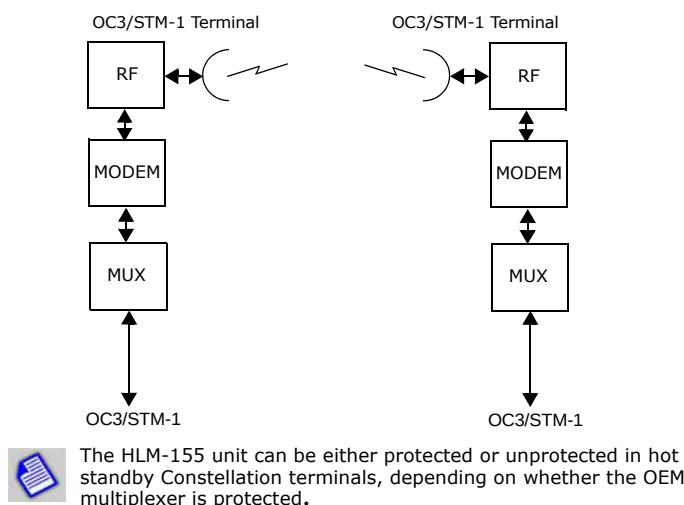
Figure 3-14: OC-3/STM-1 to OC-3/STM-1 Configuration
