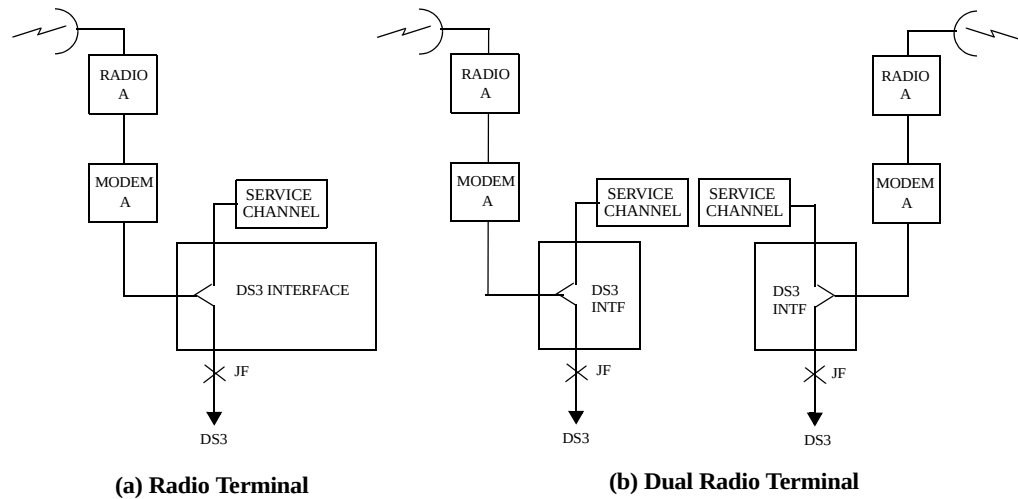
Figure 3-5: Constellation radio terminal, DS3 interface
