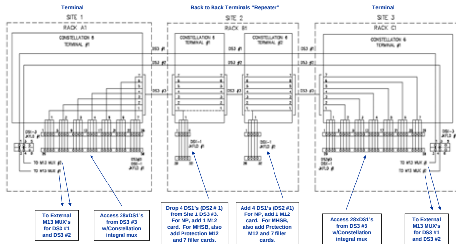
Figure 3-1: Traffic Plan Example for 3xDS3 (2xDS3+28 DS1)
