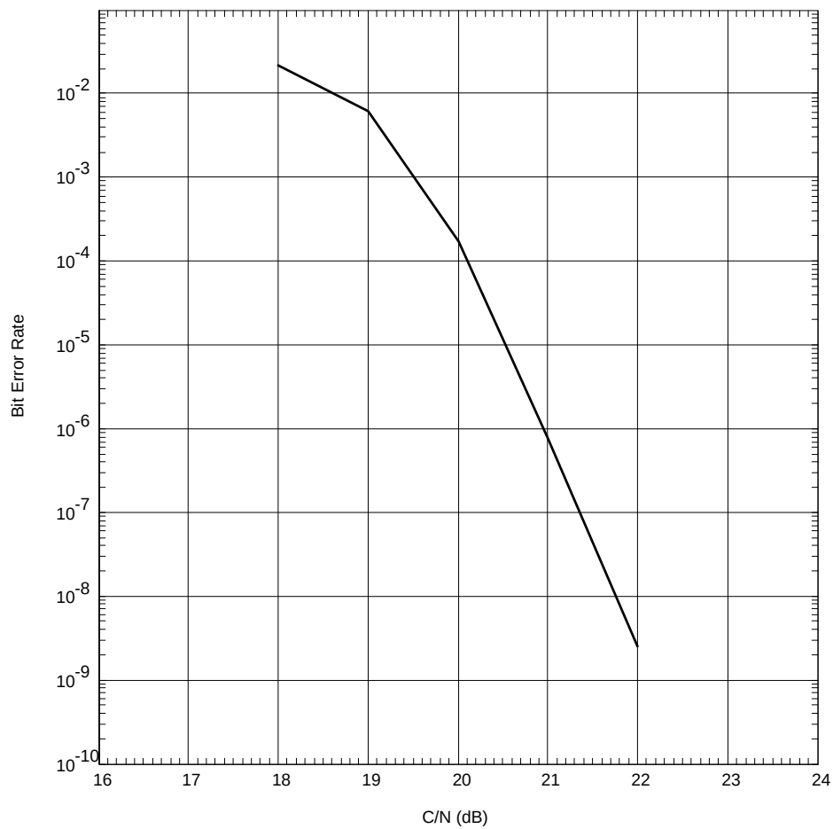
Figure 7-9: Typical BER versus C/N curve (8 DS1)
