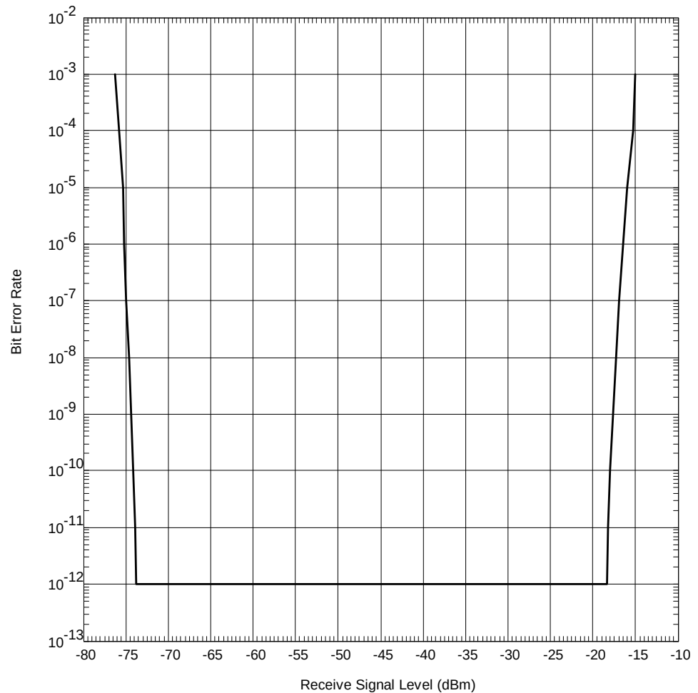
Figure 7-14: Typical BER versus RSL curve
