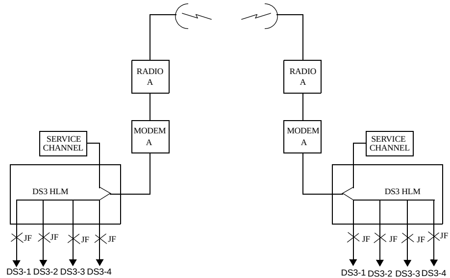
Figure 3-8: 4xDS3 to 4xDS3 configuration
