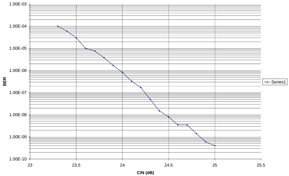
Figure 7-12: Typical BER versus C/N curve (Constellation 155)
