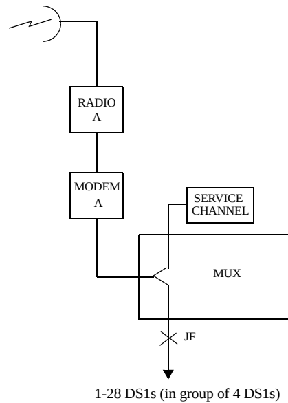
Figure 3-2: Multiplexer configuration for a radio terminal
