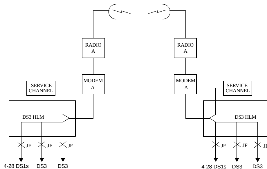
Figure 3-11: 3xDS3 configured as a 2xDS3 + 28DS1 configuration
