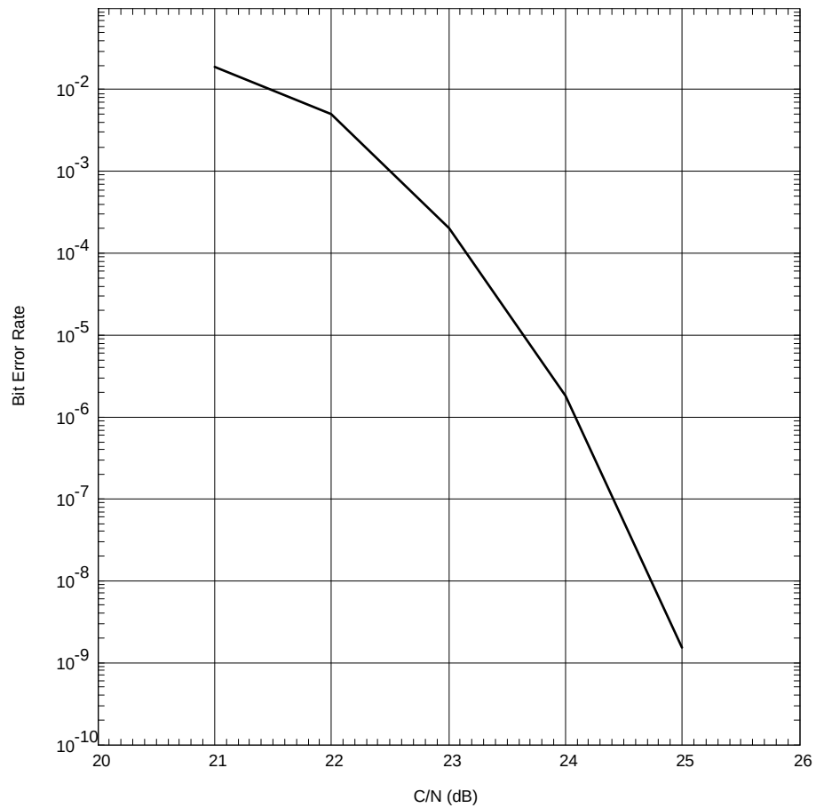
Figure 7-11: Typical BER versus C/N curve (28 DS1/DS3)
