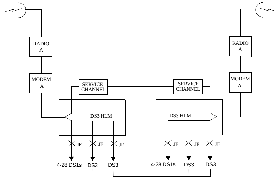
Figure 3-13: 3(4)xDS3 configured as 2(3)xDS3 + 28DS1 terminal, ADM repeater, and 3(4)xDS3 terminal
