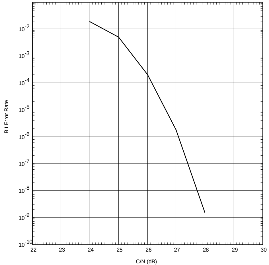
Figure 7-10: Typical BER versus C/N curve (16 DS1)
