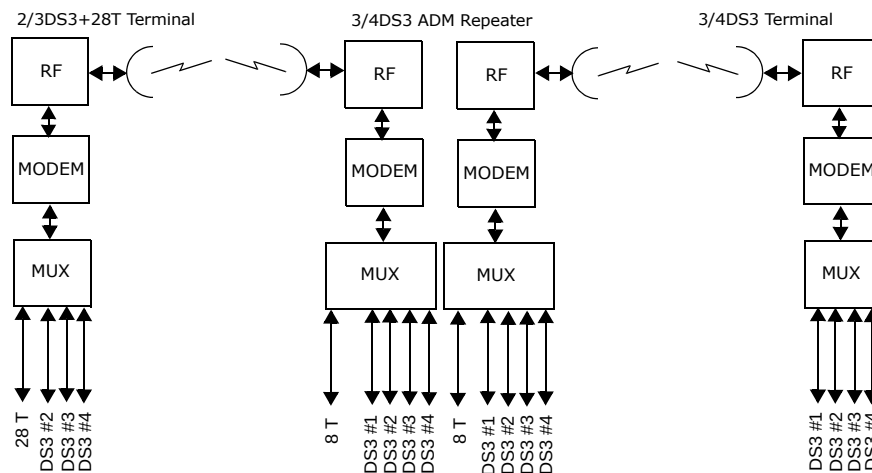
Figure 3-13: 3(4)xDS3 configured as 2(3)xDS3 + 28DS1 terminal, ADM repeater, and 3(4)xDS3 terminal
