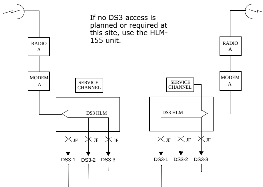
Figure 3-10: 3xDS3 to 3xDS3 back-to-back terminals
