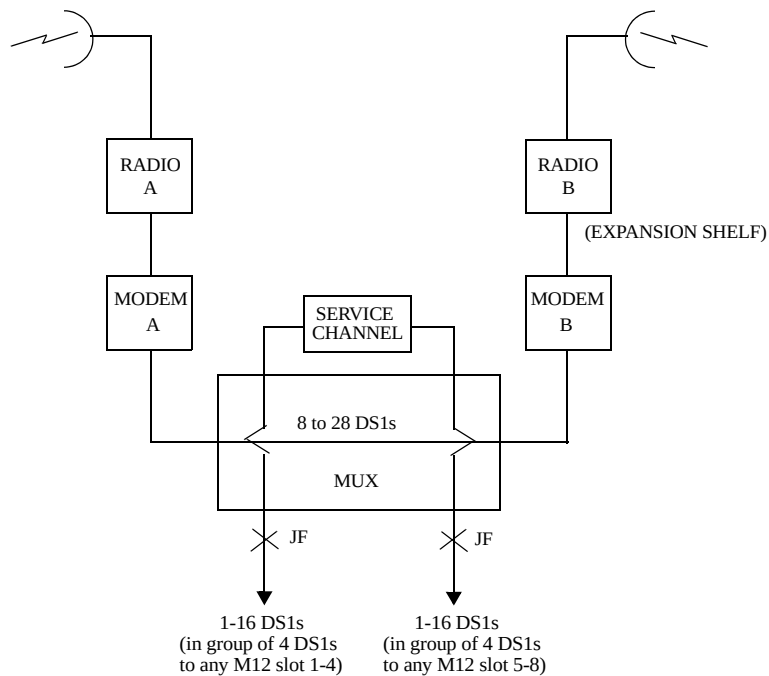
Figure 3-3: Multiplexer configuration for a radio-to-radio repeater
