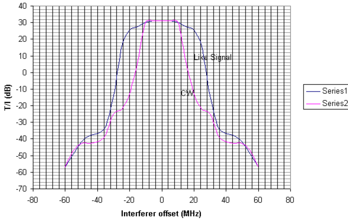
Figure 7-7: Typical threshold-to-interference (T/I) curve (6, 7/8, 10/11 GHz, 155 Mbit/s, 128 TCM)
