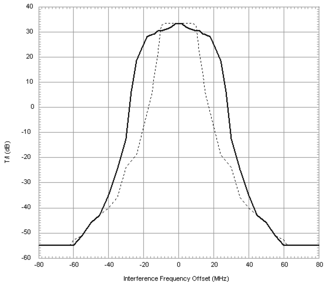
Figure 7-8: Typical threshold-to-interference (T/I) curve (6, 7/8, 10/11 GHz, 4DS3)
