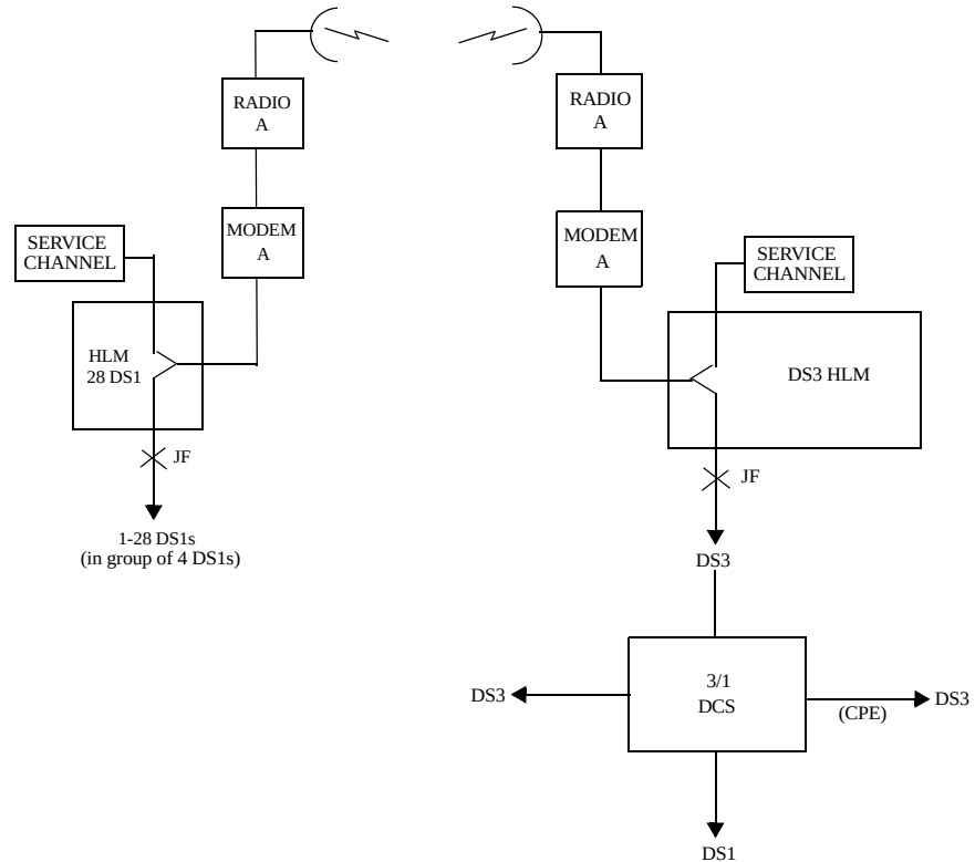
Figure 3-6: 28 DS1 to DS3 application
