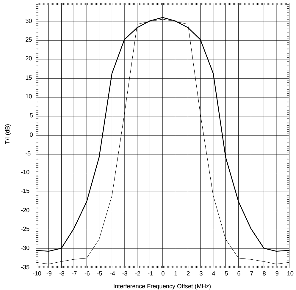
Figure 7-4: Typical threshold-to-interference (T/I) curve (10/11 GHz, 16 DS1)
