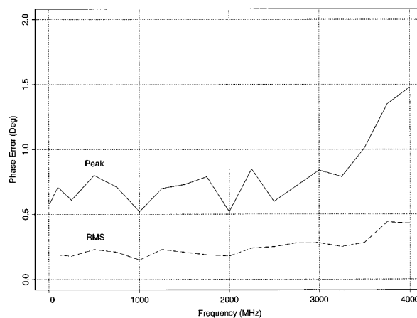
Phase error versus frequency (Gaussian filter, BbT = 0.5 , symbol rate = 1Msym/s)
