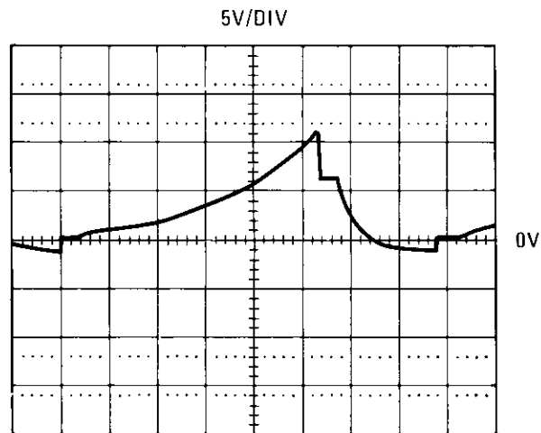
Figure 8-45. DLY/EXP Compensation (A6TP6)
