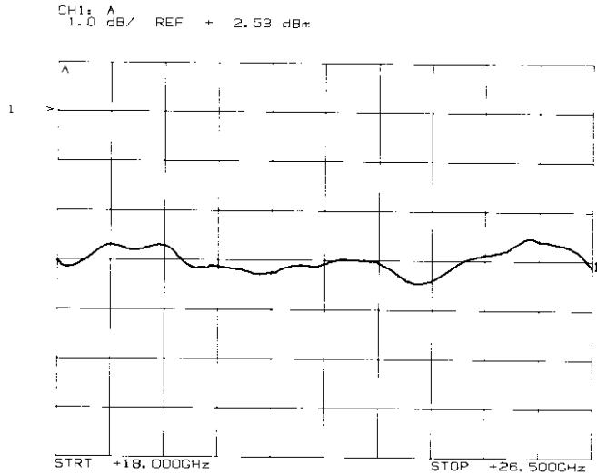
Figure 5-20. Identifying Breakpoint
