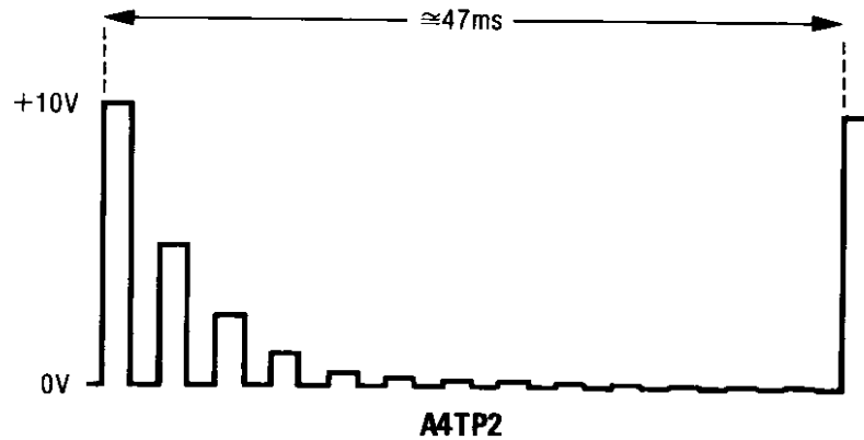
Figure 8-26. DAC Test
