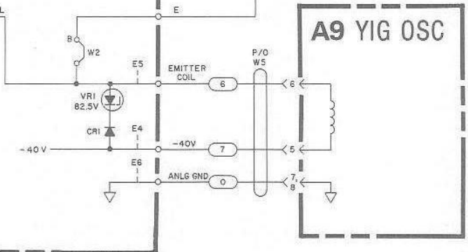
Figure 8-51. A6 YO Driver, Schematic Diagram
