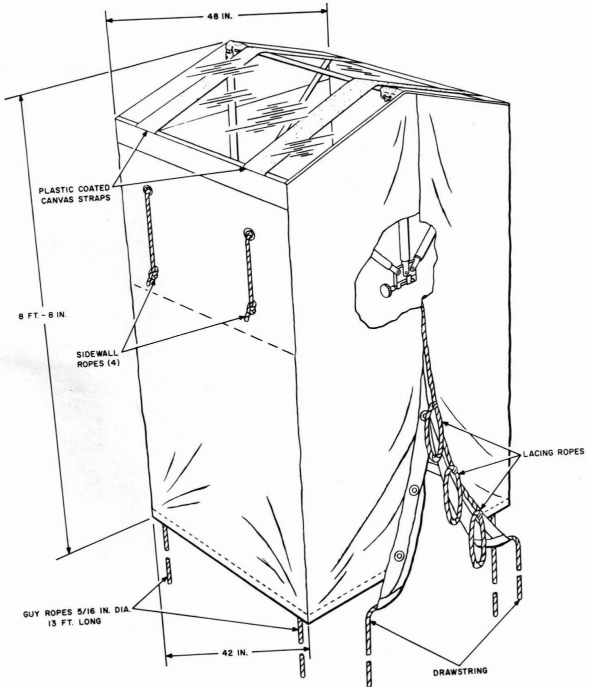
Fig. 16—Superseded C Workman's Tent
