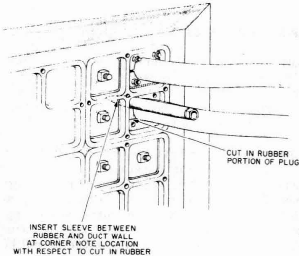
Fig. 7—Inserting Remover Sleeve
