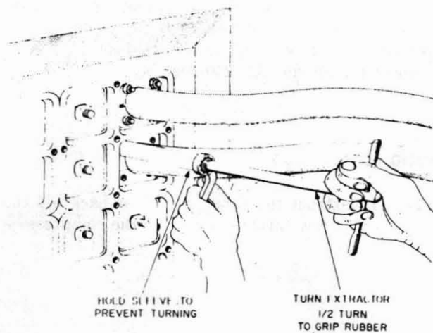
Fig. 9—Engaging Rubber with Extractor
