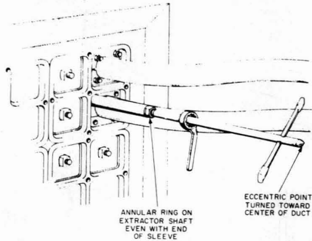
Fig. 8—Inserting Extractor
